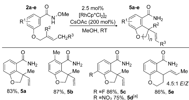
Scheme 4. \text{Rh}^{\text{III}} -catalyzed intramolecular DH-type reactions. Reaction conditions: [\text{RhCp}^*\text{Cl}_2]_2 (2.5 mol%), CsOAc (2 equiv), MeOH (0.2 M), 1–2 h. [a] 20 h reaction time.
