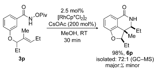
Scheme 8. Diastereoselective cyclization. Reaction conditions: see Scheme 5.
