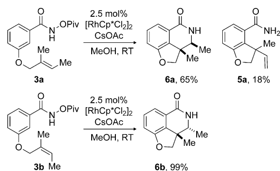
Scheme 5. Amidoarylations of E and Z olefins. Reaction conditions: [\text{RhCp}^*\text{Cl}_2]_2 (2.5 mol%), CsOAc (2 equiv), MeOH (0.2 M).
